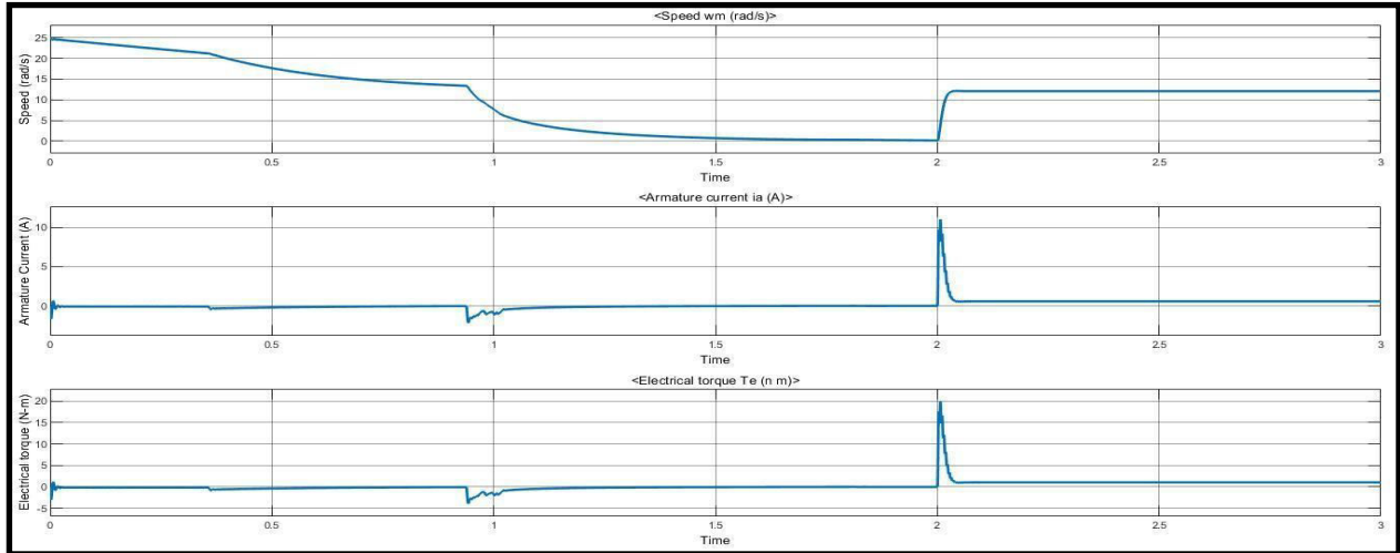
Fig 5. motor speed, Armature current, Electromagnetic torque
